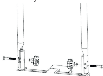
Figure 2: Assembly of U-shaped bracket
