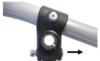
Figure 3a: Remove the carriage bolt
