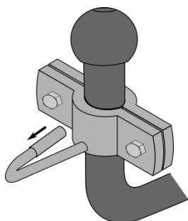
Figure 3: Pulling back the spring sleeve
