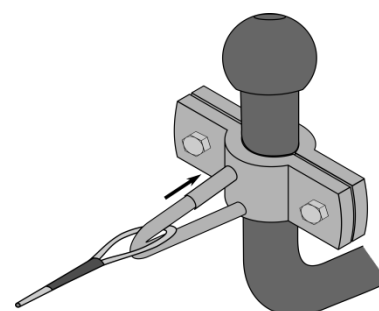
Figure 5: Closing the spring sleeve
