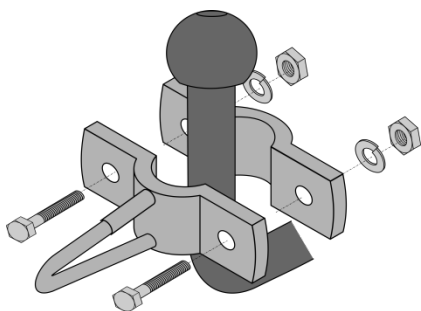
Figure 1: Individual components
