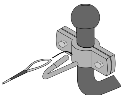
Figure 4: Mounting the breakaway cable
