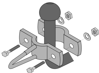
Figure 1 : Composants
